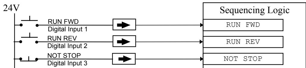
Figure 4-14 Wiring for Three Wire Logic Starting
