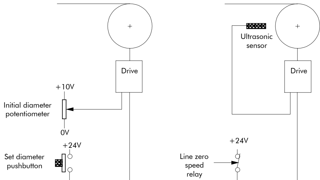
Figure 10-3 Roll Diameter
