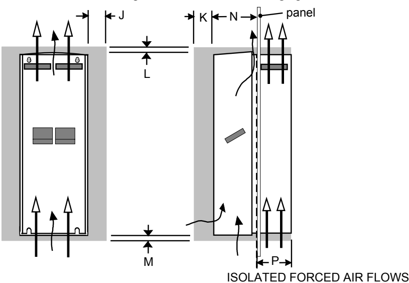
Figure 3-12 Air Clearance for a Through-Panel Mount Product/Application
