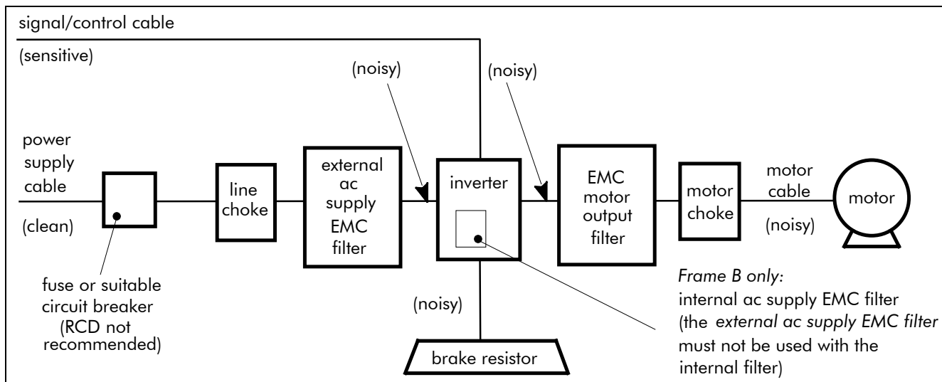
Figure 3-14 Cabling Requirements
