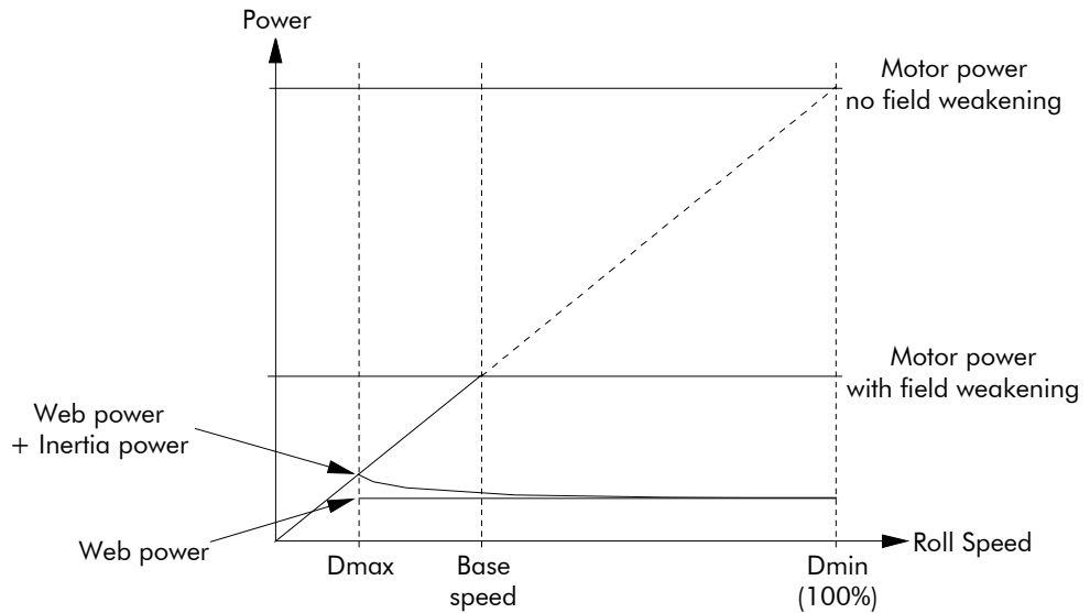
Figure 10-7 Motor Power
